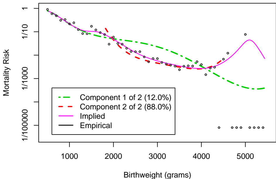
(c) Estimated mortality in 2-component model
