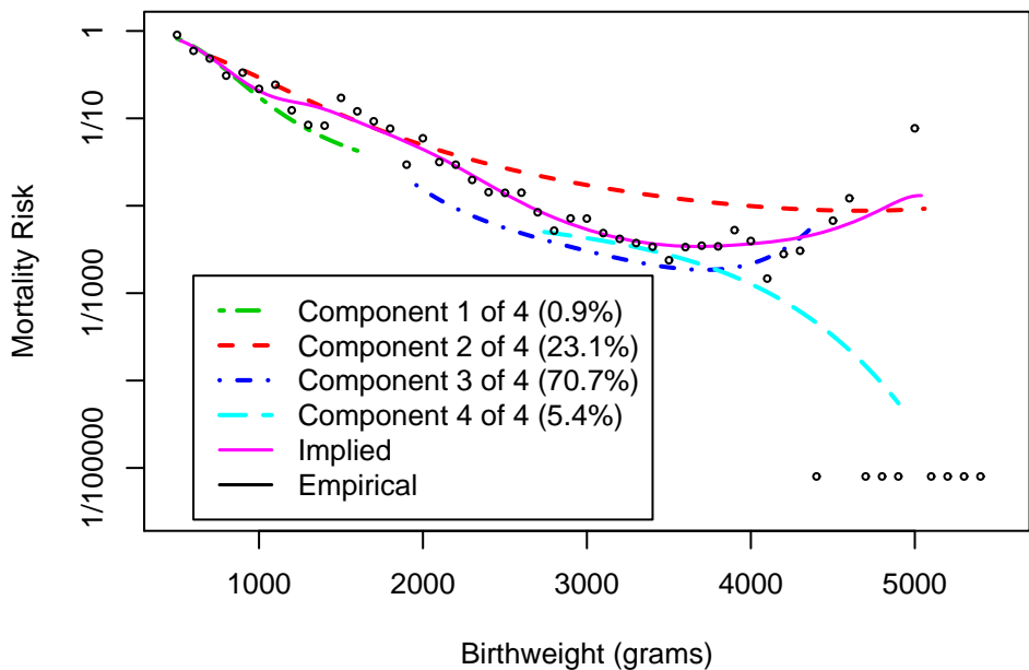
(a) Estimated mortality in 4-component model
