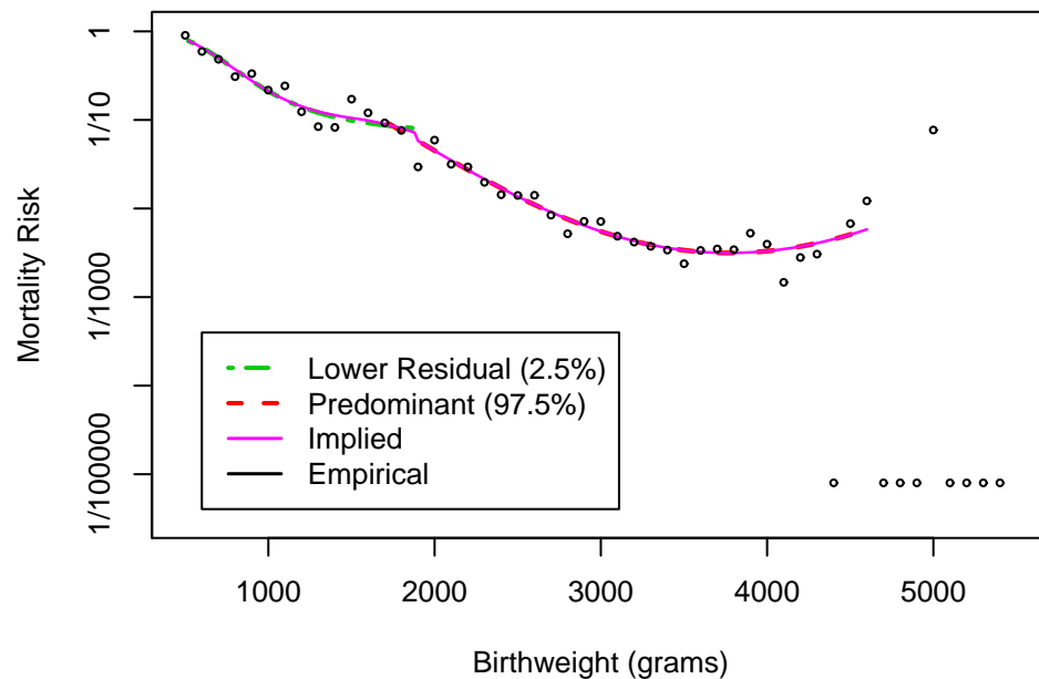
(b) Estimated mortality in contaminated model
