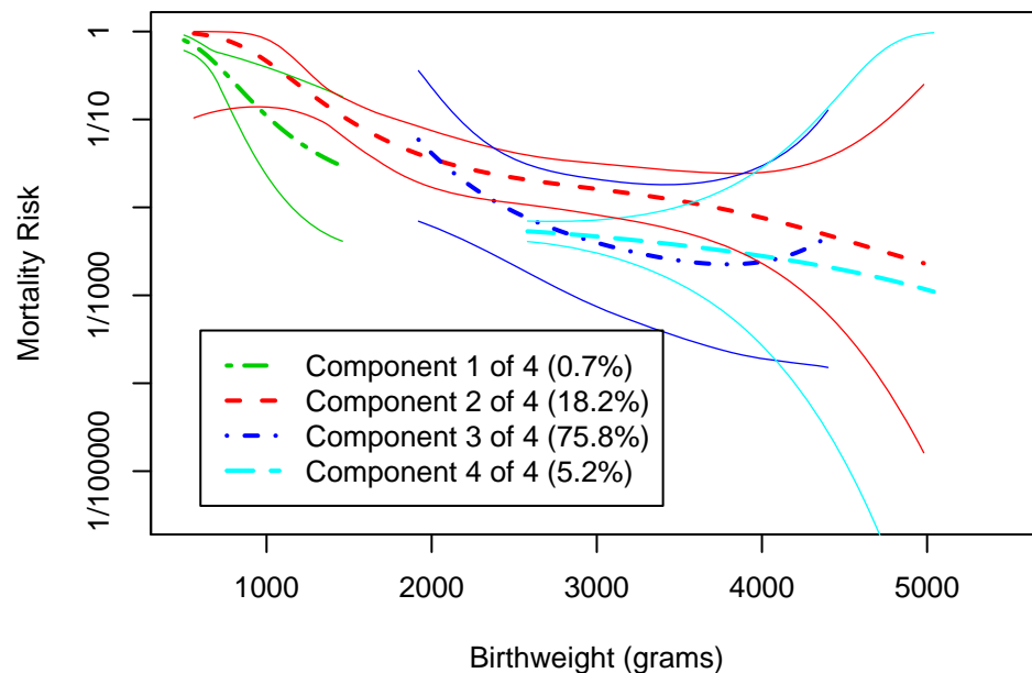
(d) Confidence bounds for mortality in 4-component model
