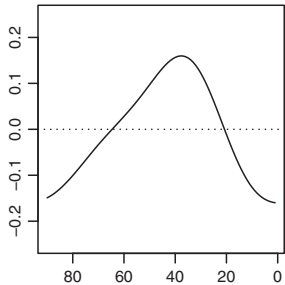
FPC3 for temporal mean
