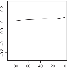
FPC1 for temporal mean
