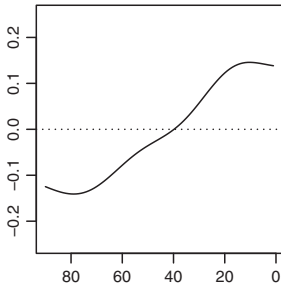
FPC2 for temporal mean
