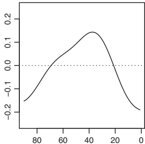
FPC3 for temporal SD
