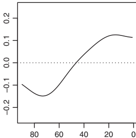
FPC2 for temporal SD
