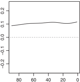
FPC1 for temporal SD
