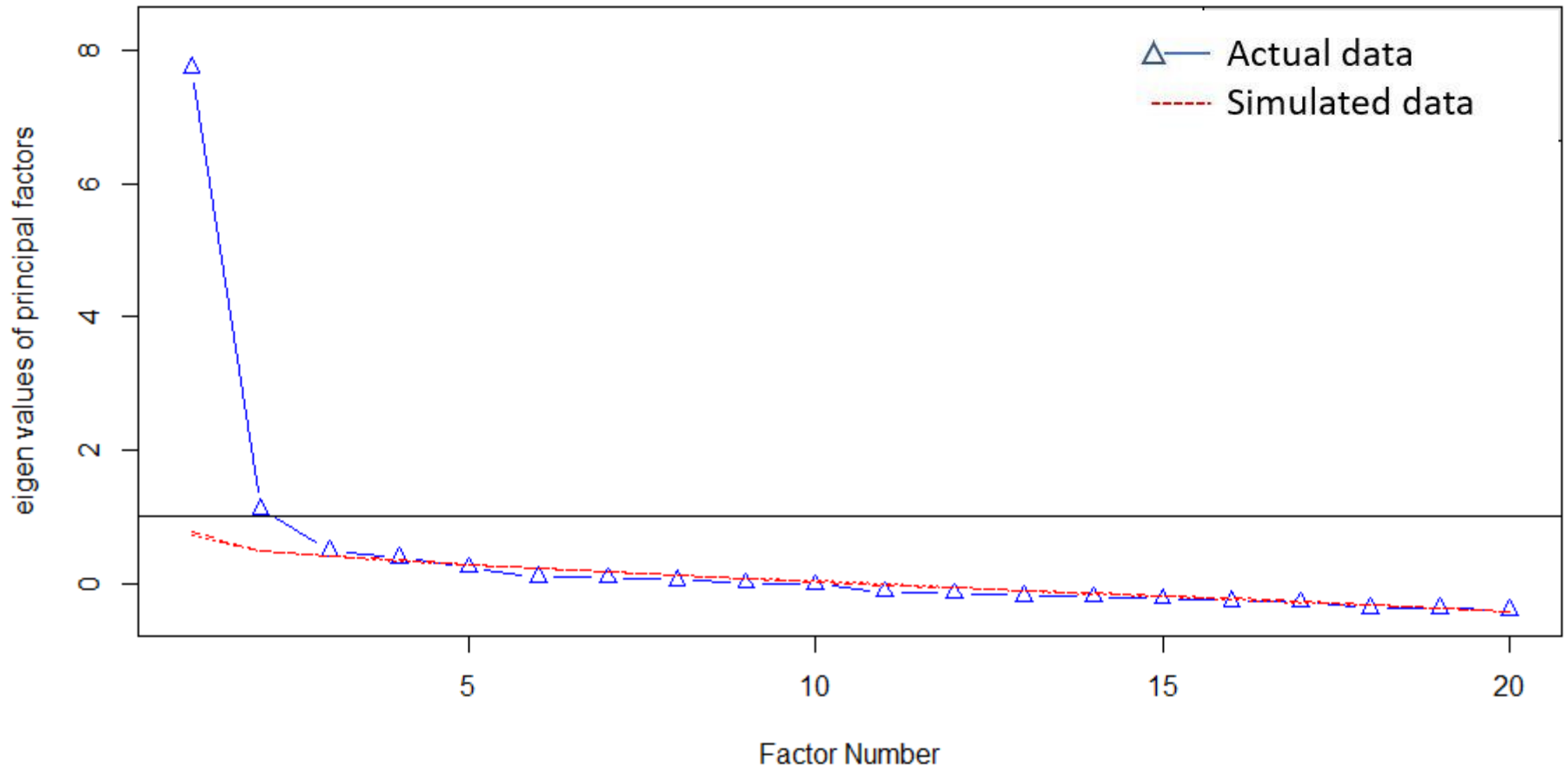
Figure 3. Scree plot following parallel analysis of the postnatal scale.
