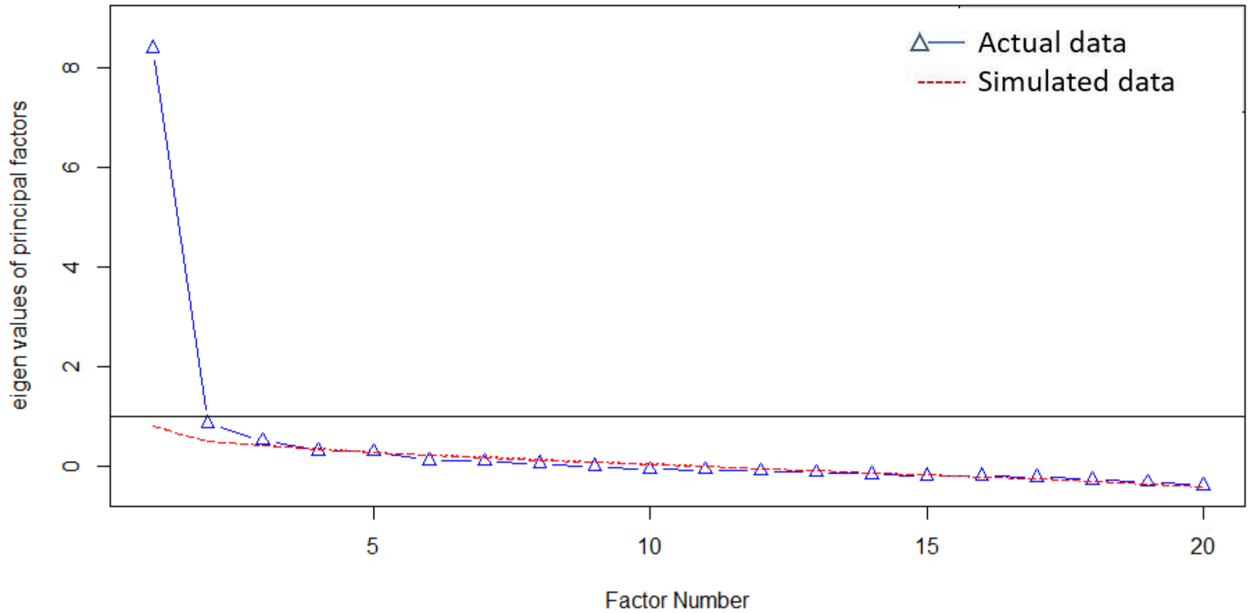
Figure 2. Scree plot following parallel analysis of the labour and childbirth scale.
