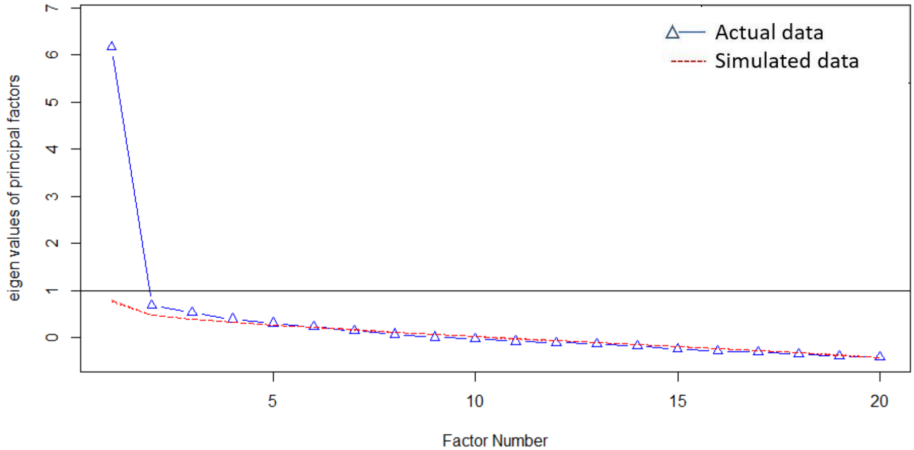
Figure 1. Scree plot following parallel analysis of the pregnancy scale.
