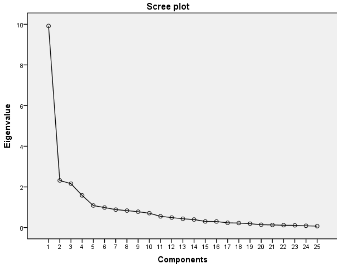
Supplementary Figure 1: A scree plot showing distribution of factors by their eigenvalues.
