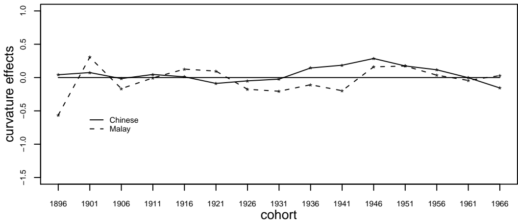
c) Cohort curvature effects
