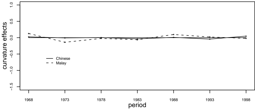
b) Period curvature effects
