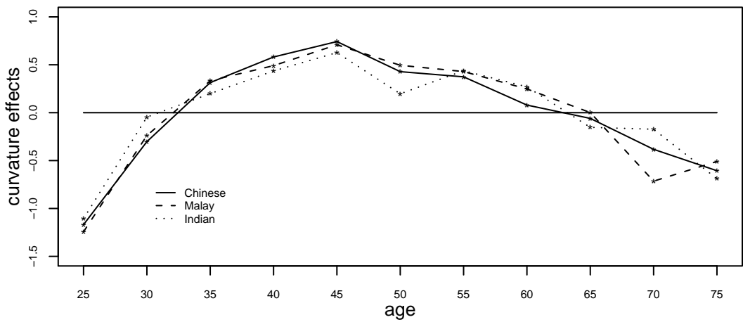
a) Age curvature effects
