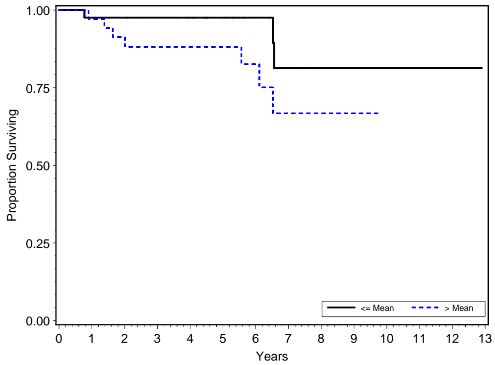
A. Development of Invasive Disease by Texture (Difference Entropy)
