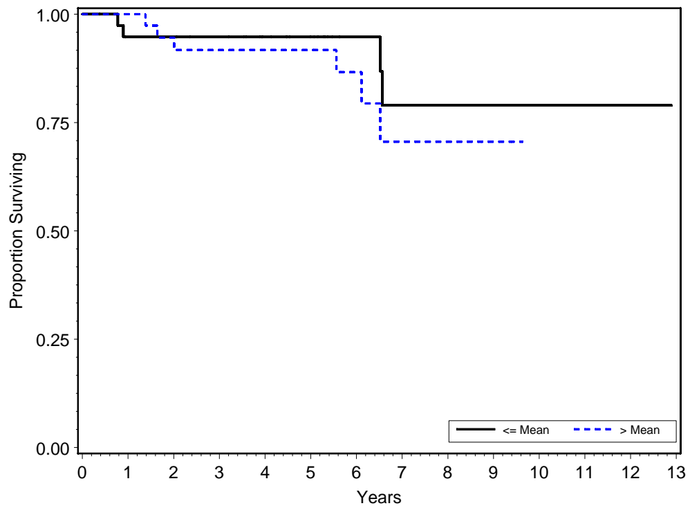
B. Development of Invasive Disease by Texture (Contrast)
