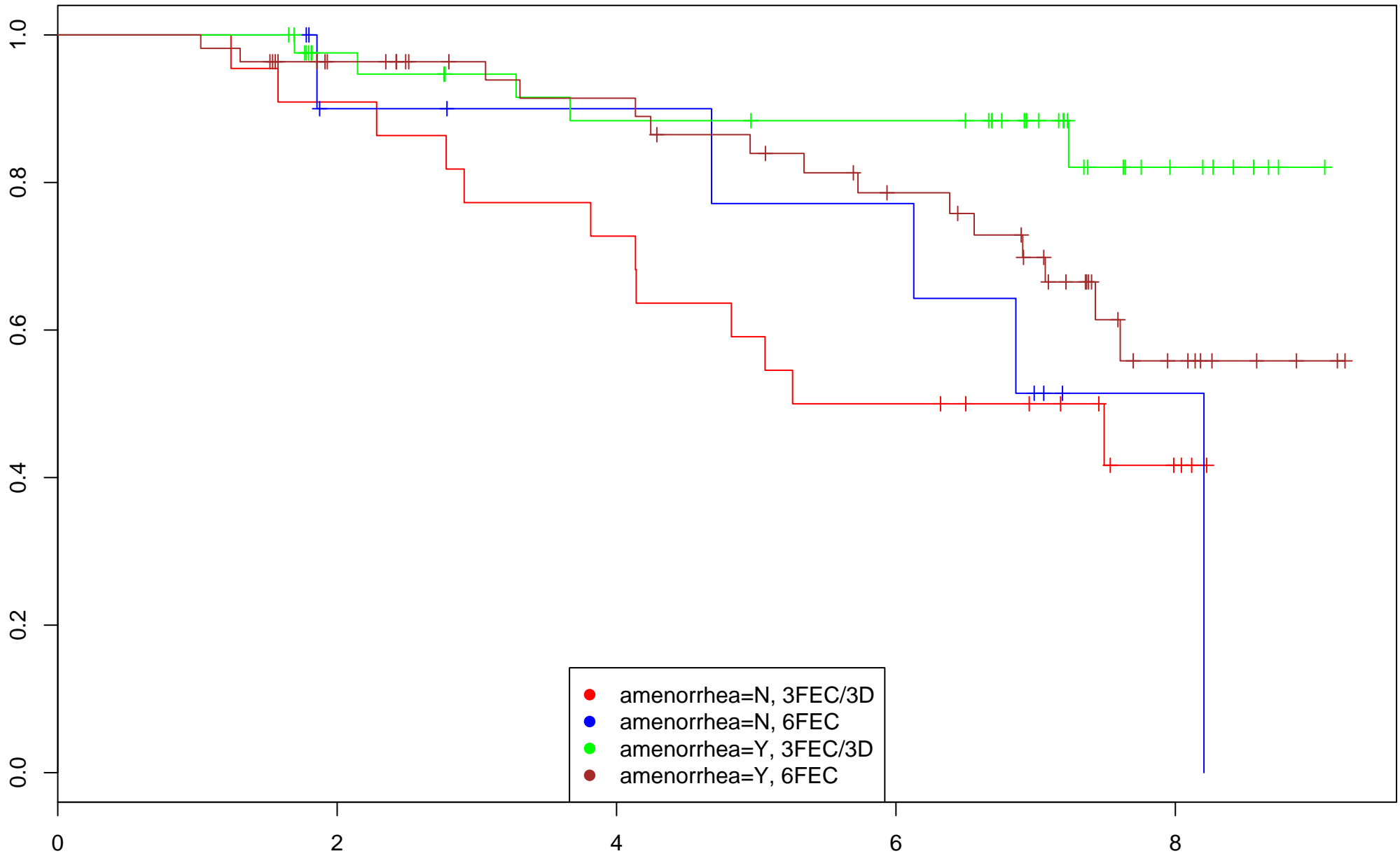
Kaplan-Meier curves
