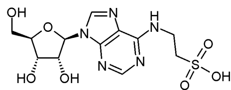
9-ribosyl-6-taurinopurine (M-4)
