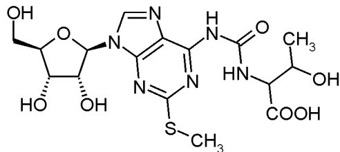
2-methylthio-N 6 -threonylcarbamoyladenine (ms 2 t 6 A)
