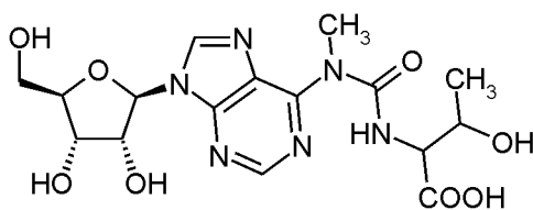
N 6 -methyl-N 6 -threonylcarbamoyladenine (m 6 t 6 A)
