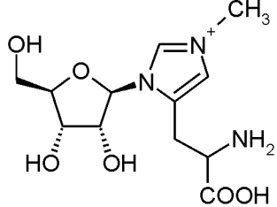
1-ribosyl-3-methyl-5-(2-amino-carboxyethyl)-imidazolium (M-1)
