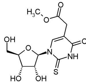
5-methoxycarbonylmethyl-2-thiouridine (mcm 5 s 2 U)
