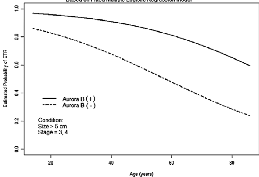
Conditional Effect Plot of Age and Aurora B on the Probability of ETR Based on Fitted Multiple Logistic Regression Model
