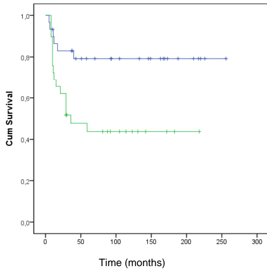
KRT19
