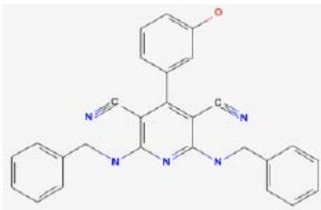
NSC 734406: 2,6-bis(benzylamino)-4-(3-hydroxyphenyl)pyridine-3,5-dicarbonitrile
