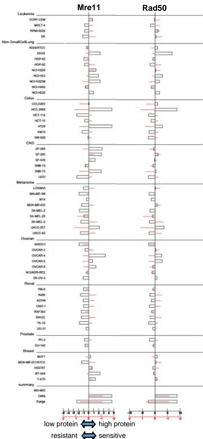
NSC 734406: 2,6-bis(benzylamino)-4-(3-hydroxyphenyl)pyridine-3,5-dicarbonitrile
