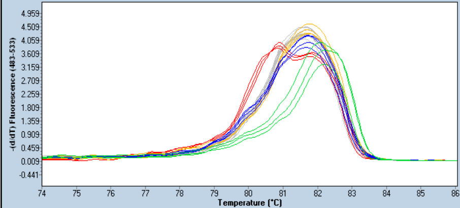
Melting Peaks
