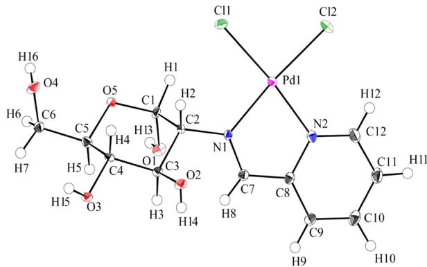
[\text{PdCl}_2(\text{L})]
