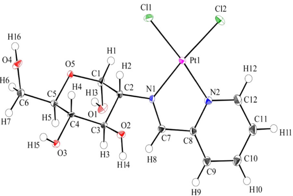
[\text{PtCl}_2(\text{L})]
