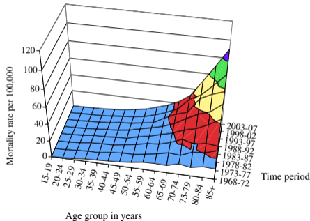
(b) Australian melanoma mortality for men
