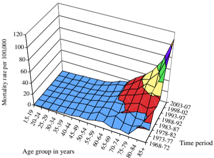
(a) New Zealand melanoma mortality for men
