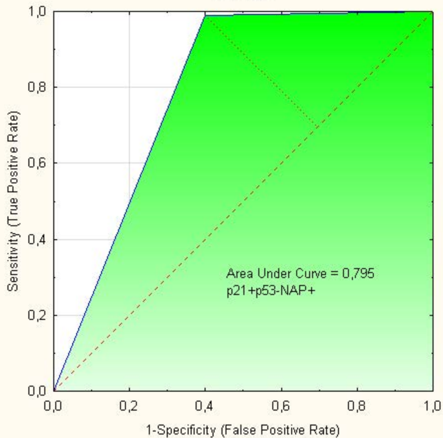
ROC Curve
