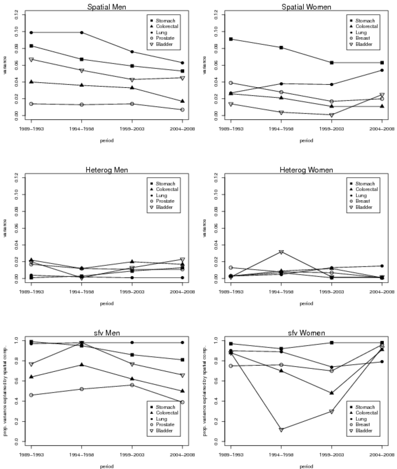
Figura-s2. Plots showing the evolution of the variance of model spatial and heterogeneity components and the proportion of the mortality relative risk variance explained by the spatial structure of the models.
