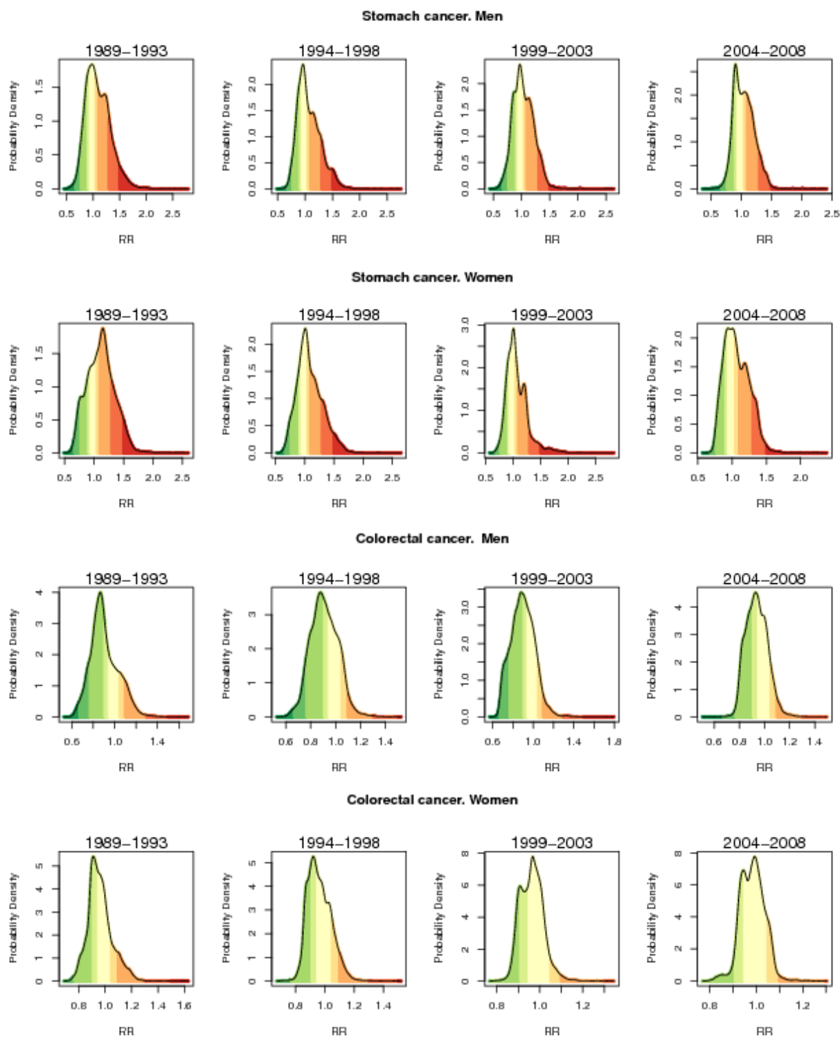
Figure-s1. Probability density functions showing distribution of smoothed relative risks used in each map
