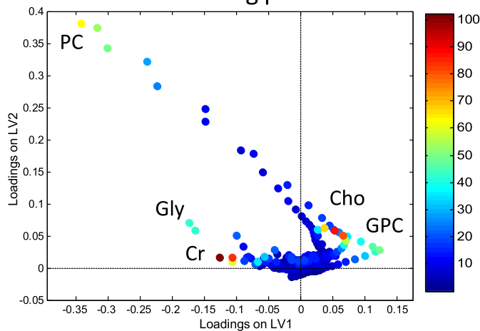
Loading plot
