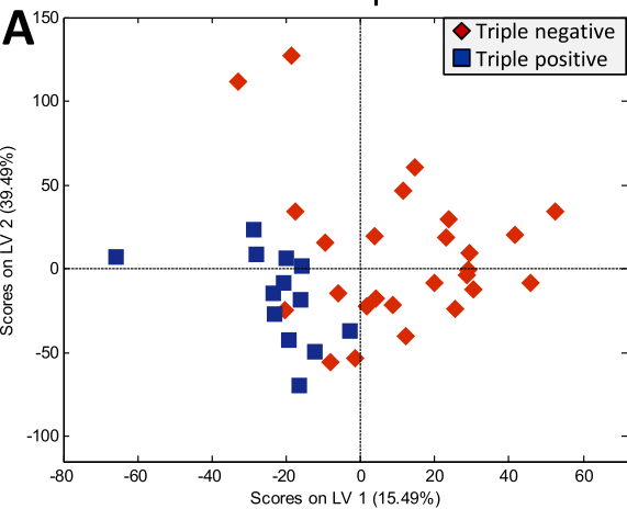
Score plot
