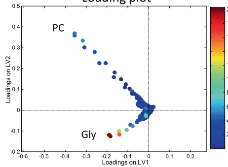
Loading plot
