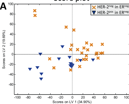
Score plot
