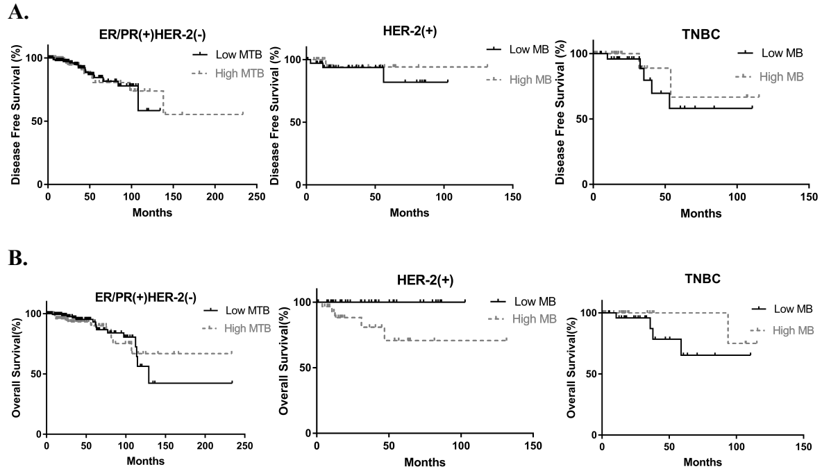
Figure S9. Kaplan-Meier estimates for high and low mutation burden. KM survival curves are shown for (A) disease-free survival and (B) overall survival between cases with high and low mutation (MB) burden, the upper and lower quartiles, in each subtype of breast cancer. Here we defined the top quartile of mutation burden as high and the bottom quartile as low.
