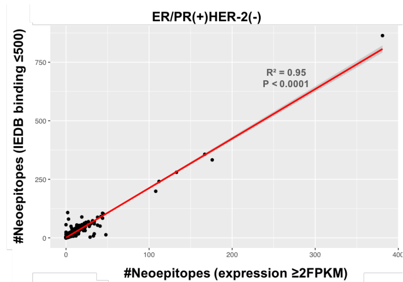
Figure S6. Correlation of number of potential binding neoepitopes with number of expressed (FPKM \geq 2) neoepitopes. The number of potential binding neoepitopes (IEDB score \leq 500) are highly correlated with the number of expressed neoepitopes (FPKM \geq 2) for all three subtypes of breast cancer. In all the plots a linear regression model is used to fit the data; the fitted line is shown in red and 95% CIs are shown in grey.
