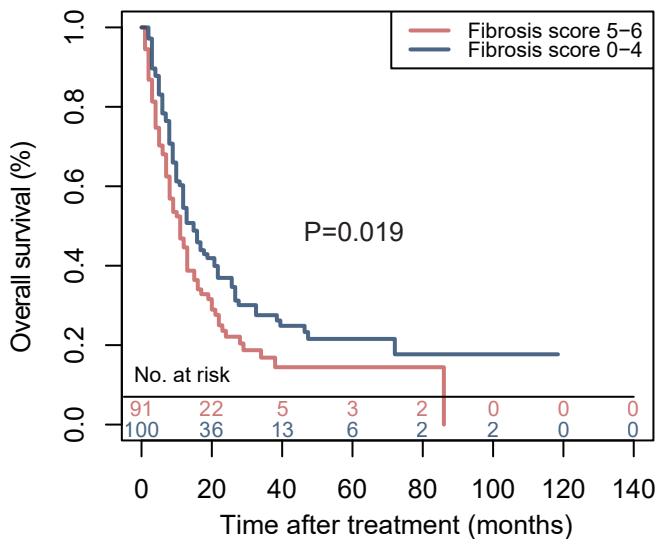
A: Kaplan-meier curve in chemotherapy patients
