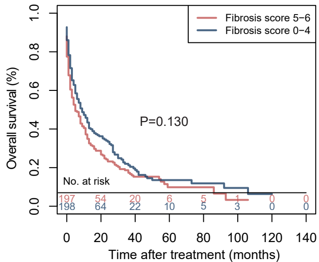
D: Kaplan-meier curve in non-radiotherapy Patients
