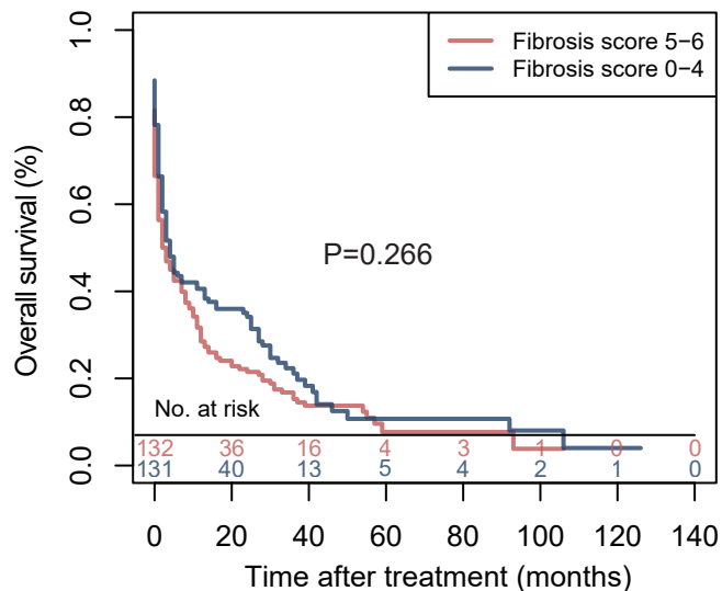
B: Kaplan-meier curve in non-chemotherapy patients
