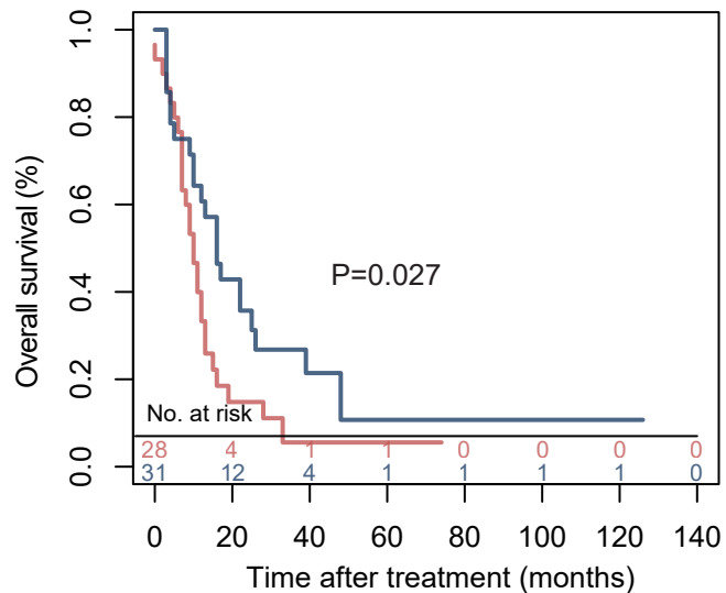
C: Kaplan-meier curve in radiotherapy patients
