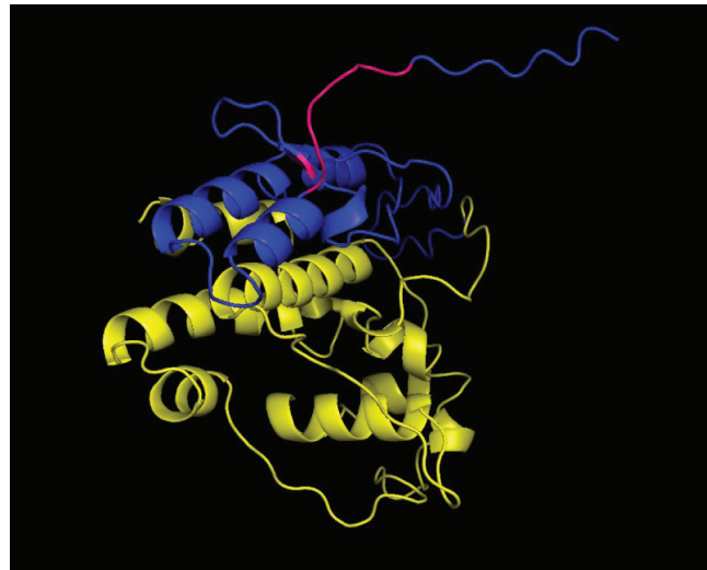
PGAP SRPK-1 Predicted Binding Site
