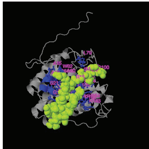
Alternative Predicted Binding Site
