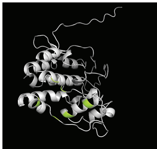
SRPK-1 Active Binding Site
