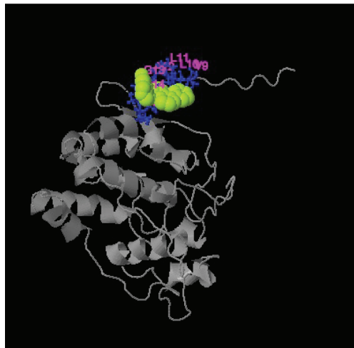
Predicted Binding Pattern
