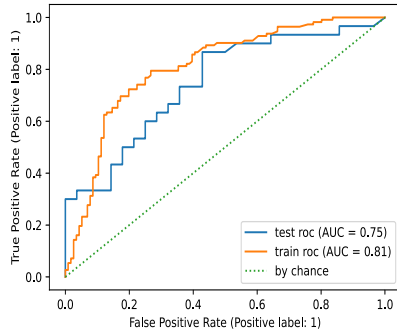
ROC on test set of GNB
