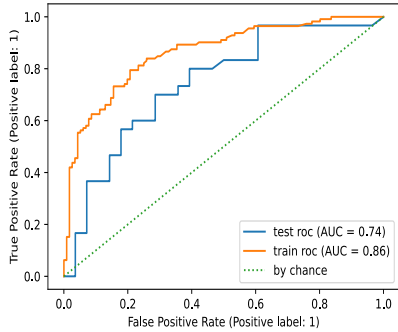
ROC on test set of ANN
