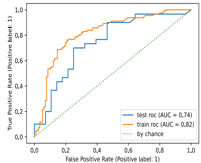
ROC on test set of SVM
