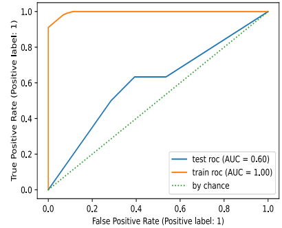
ROC on test set of Decision Tree
