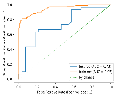
ROC on test set of CatBoost
