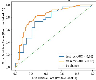
ROC on test set of Logistic
