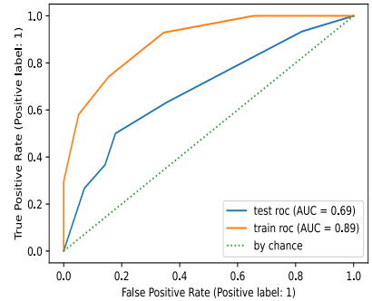
ROC on test set of KNN
