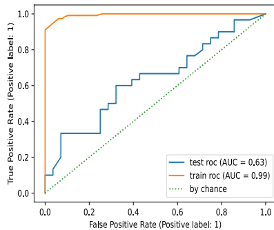
ROC on test set of Random Forest
