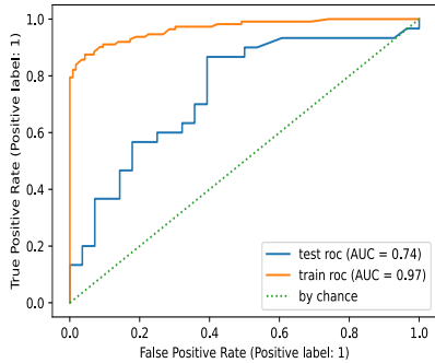
ROC on test set of GBM
