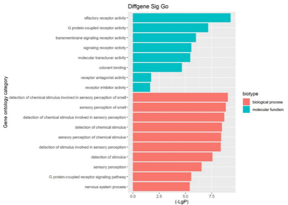
Figure S2. GO Enrichment Analysis (Group B versus Group C). A: upregulated transcripts; B: downregulated transcripts. The x-axis shows -\log_{10}(P\text{-value}) . The y-axis shows GO category. P < 0.05 was considered to be statistically significant. Group B consisted of patients with PDR pretreated with coberccept 3–7 days before surgery; Group C consisted of patients with PDR who underwent surgery alone. GO: Gene Ontology; PDR, proliferative diabetic retinopathy.
