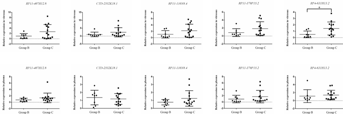
Figure S5. Expression levels of lncRNAs of the confirmation cohort, in vitreous and plasma (Group B versus Group C). The levels of lncRNAs were determined by qRT-PCR. The data of each group are expressed as the relative expression. The asterisk indicates the significant difference. Group B consisted of patients with PDR pretreated with conbercept 3–7 days before surgery; Group C consisted of patients with PDR who underwent surgery alone. qRT-PCR, quantitative real-time polymerase chain reaction; PDR, proliferative diabetic retinopathy.
