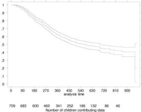
Kaplan-Meier survival estimate 95% pointwise confidence band show n
