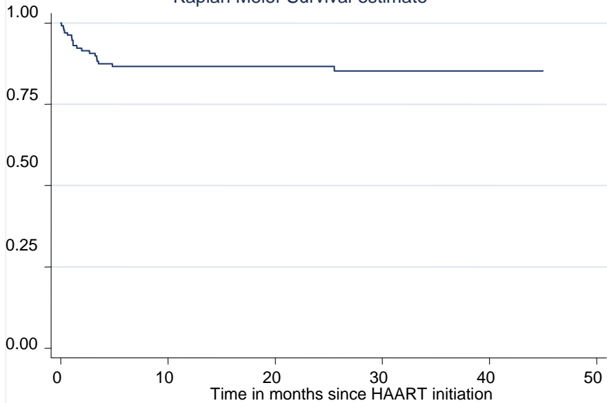
Kaplan Meier Survival estimate
