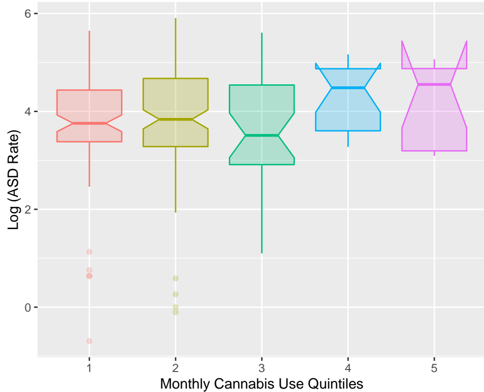
Log (ASD Rate) by Quintiles – All Data
