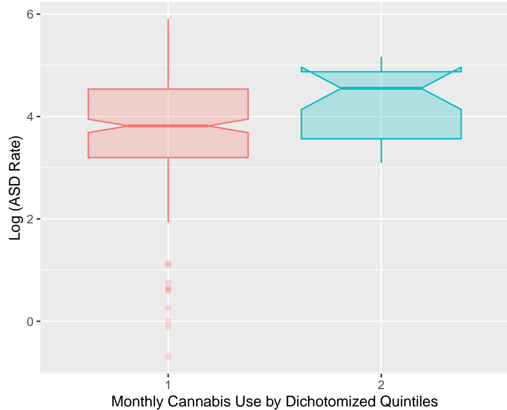
Log (ASD Rate) by Quintiles 1, 2 & 3 Vs. Quintiles 4 & 5 – All Data
