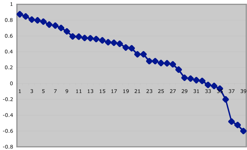
Promax Component 1 Loadings
