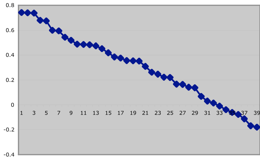
Promax Component 2 Loadings
