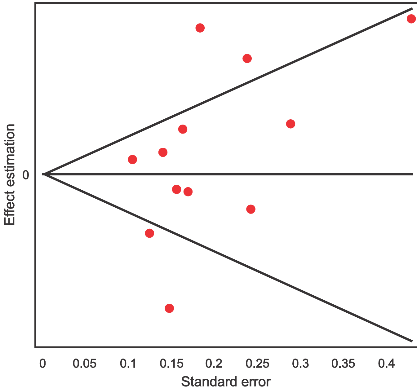
Funnel plot
