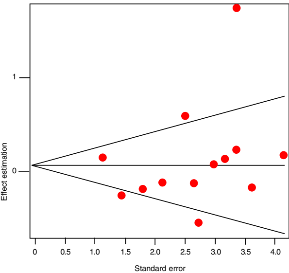
Funnel plot
