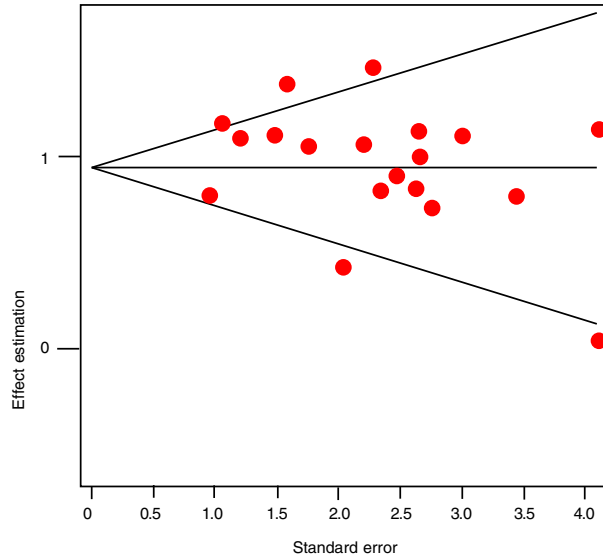
Funnel plot
