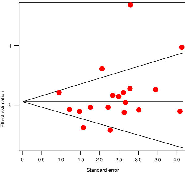
Funnel plot
