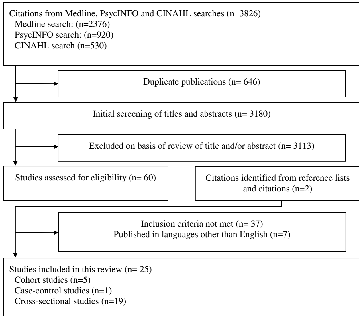
Figure 3: Summary of systematic search presented as an adapted CONSORT diagram
