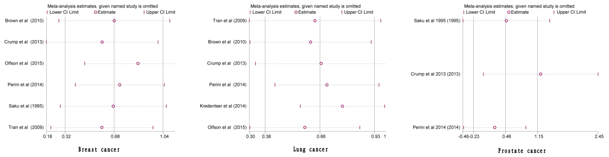
Fig. S2 Metaninf test of studies included in meta-analysis of breast, lung and prostate cancer
