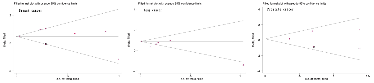
Fig. S1 Metatrim test of studies included in meta-analysis of breast, lung and prostate cancer
