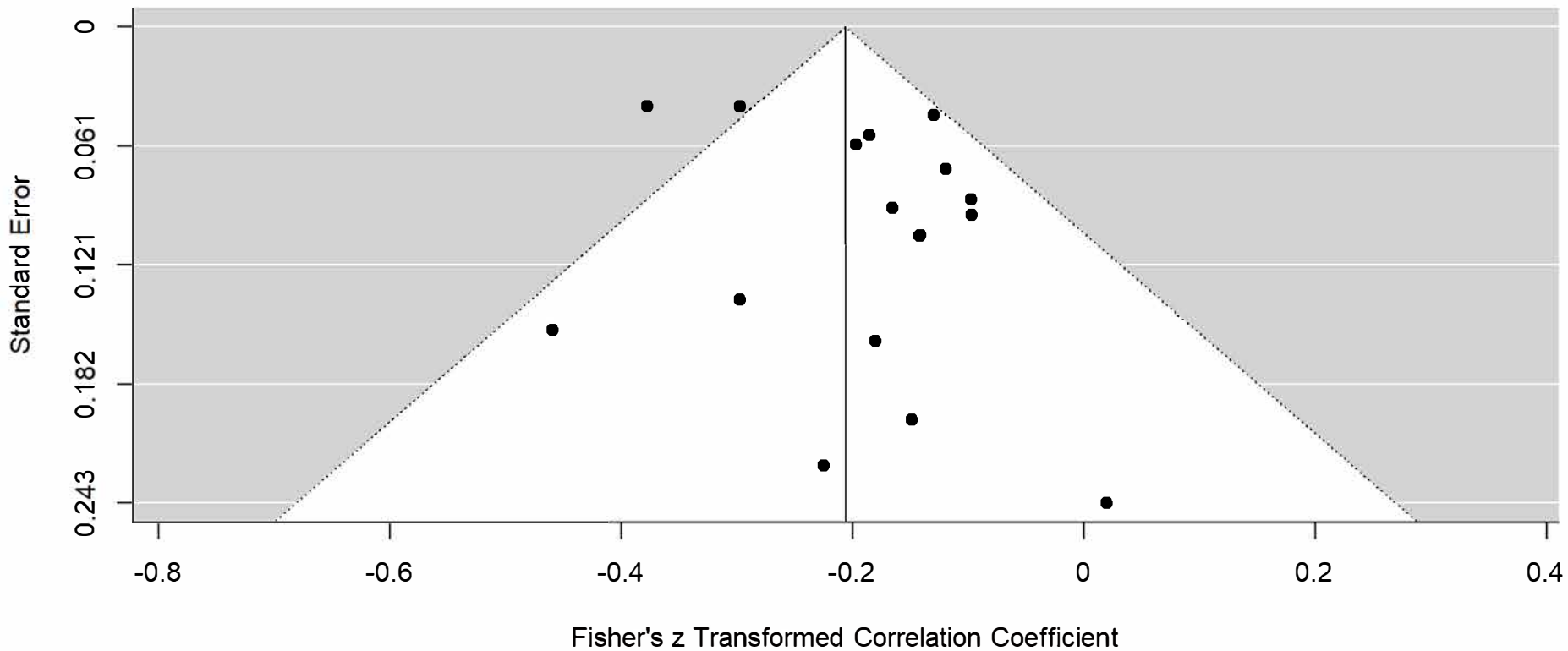
Additional File 5. Funnel plot for the meta-analysis of uncorrected partial correlations.
