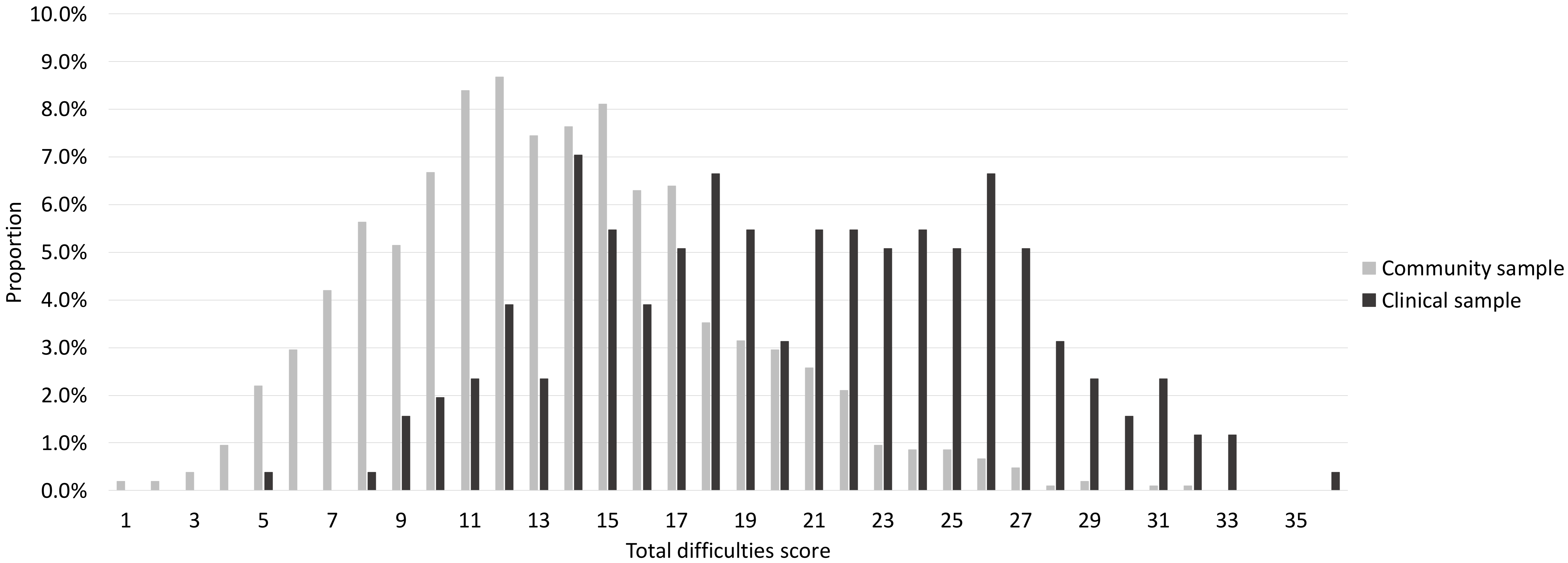
Distribution of total difficulties score (Male participants)
