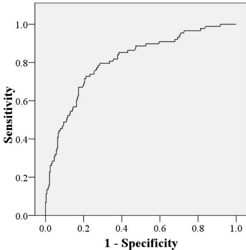
ROC Curve
