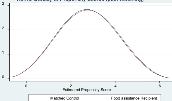
Kernel Density of Propensity Scores (post-Matching)
