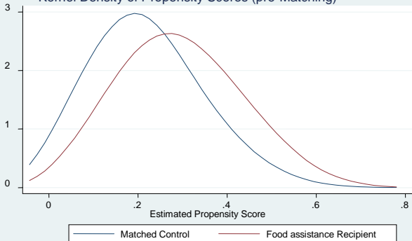
Kernel Density of Propensity Scores (pre-Matching)
