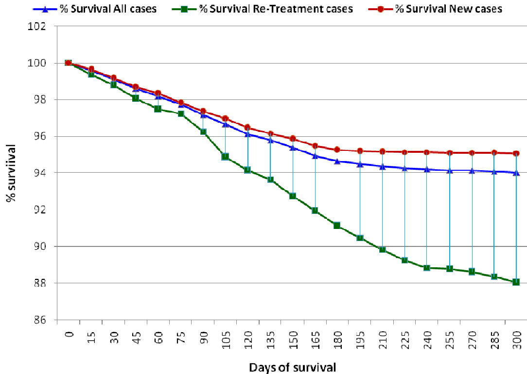
Survival curves for TB cases (7012 New, 1228 Retreatment cases)
