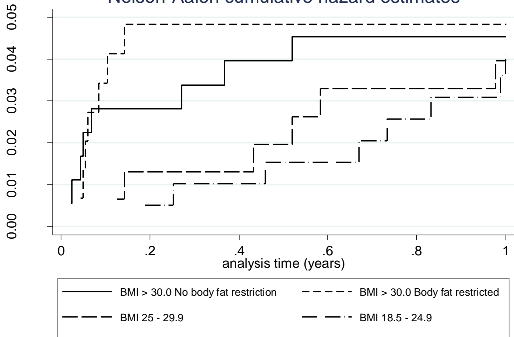
Nelson-Aalen cumulative hazard estimates
