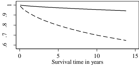
Survival function
