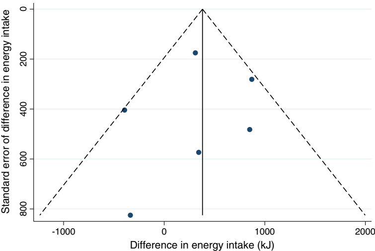
Funnel plot with pseudo 95% confidence limits
