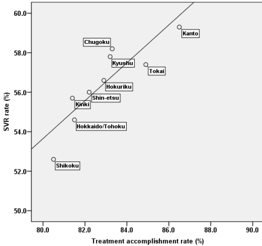
Additional Figure 1. Correlation between treatment accomplishment and sustained virological response (SVR) rates in patients treated by peginterferon- \alpha and ribavirin in nine regions of Japan. SVR rates were strongly correlated with the rates of treatment accomplishment ( r = 0.879 , P = 0.002 ).
