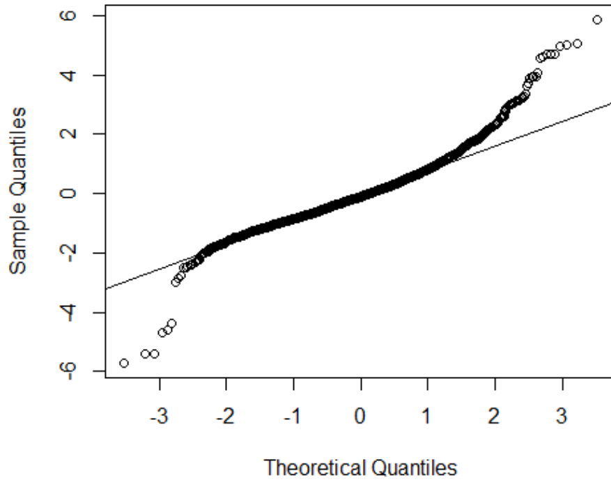
Normal Q-Q Plot
