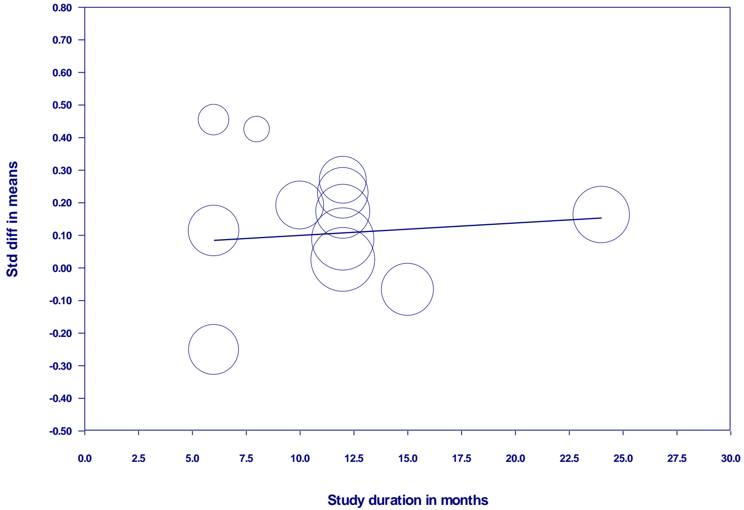
Regression of Std diff in means on Study duration in months
