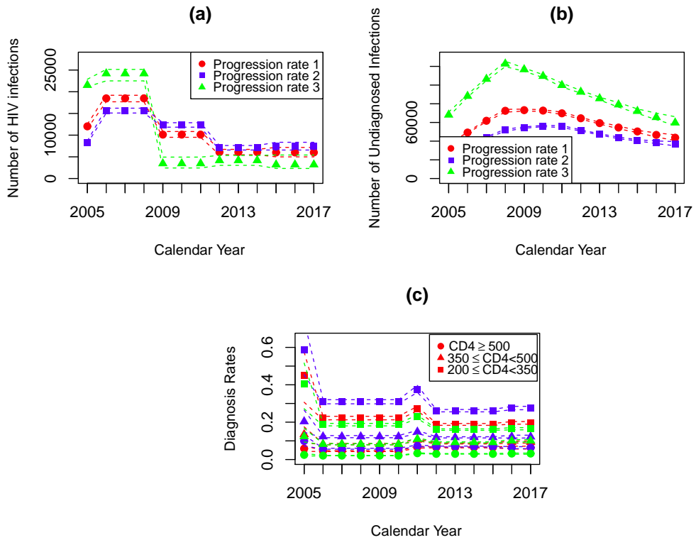
Fig. S4: The comparison of new infections (a), undiagnosed infections (b), and diagnosis rates (c) by three different groups of progression rates (estimated by method 2). The waiting time in each CD4 stage for red, blue and green are PR1:3, 3, 3; PR2: 2.56, 2.17, 2.16 and PR3: 6.37, 2.86 3.54, respectively. The dotted lines give the 95% CI.
