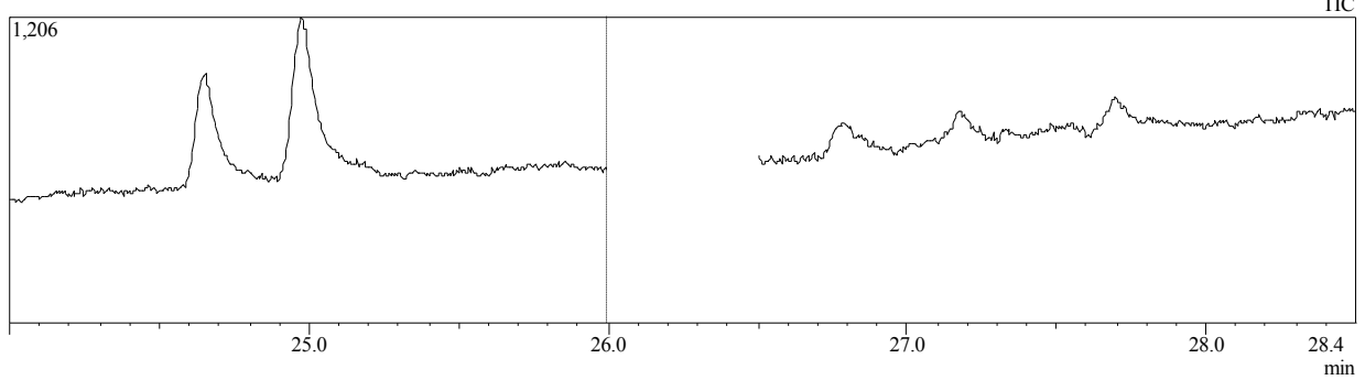
Chromatogram 13082019_mary_500ppb_rep C:\GCMSsolution\Data\Project1\13082019_mary_500ppb_rep001.qgd
