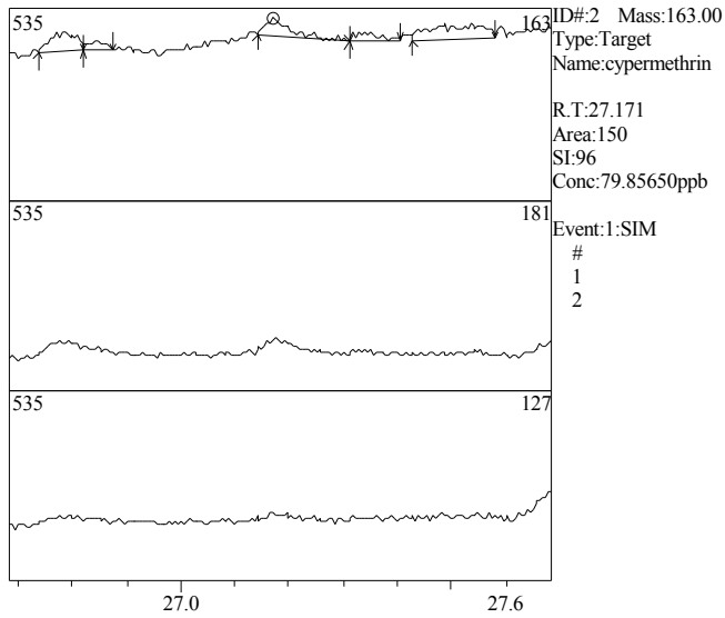
Chromatogram 13082019_mary_500ppb_rep C:\GCMSsolution\Data\Project1\13082019_mary_500ppb_rep001.qgd
