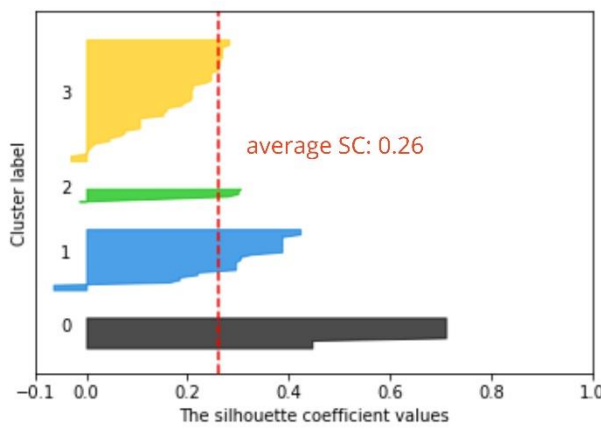
4 clusters
