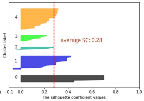
5 clusters
