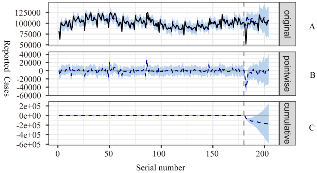
Fig. S1 Time series plot of causal effects of the COVID-19 on hepatitis B notifications in 2020-2021. The panel A, B and C shows the hepatitis B case notifications and counterfactual forecasted results for the post-outbreak period, pointwise causal effect and cumulative effect respectively.
