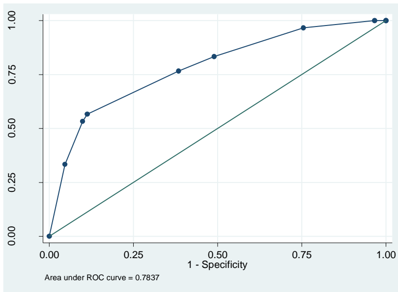
Figure 2. Results from validation of the CART model – ROC Curve
