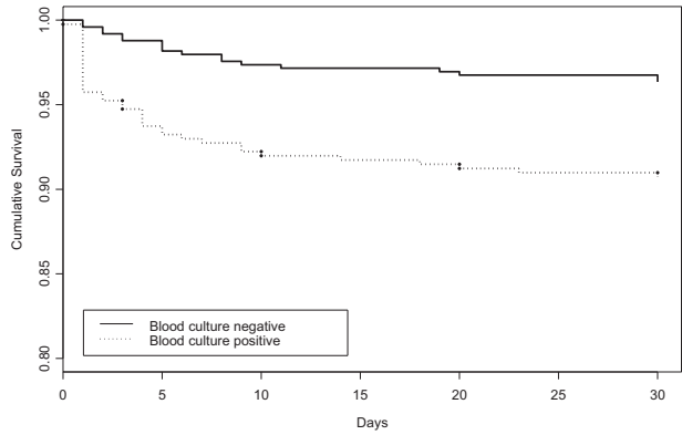
Survival Functions: 30-day mortality
