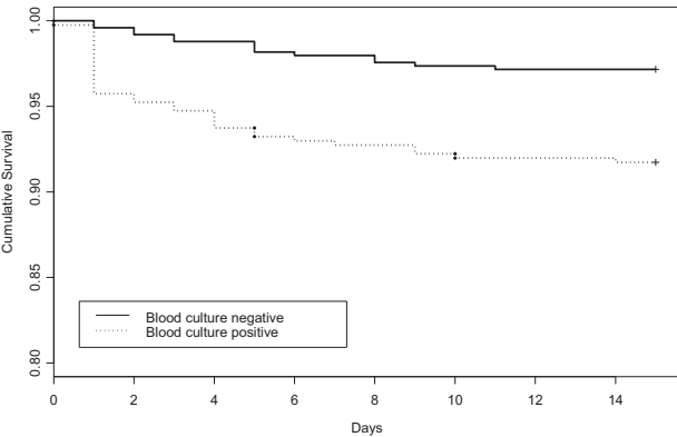
Survival Functions: 15-day mortality
